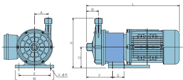
TS-71PH/71VH (ネジ接続)
